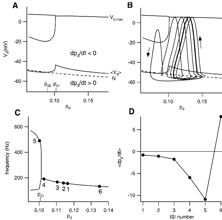
Figure 9. A: The bifurcation diagram of Fig. 6A is replotted along with the p_d nullcline p_{d,\infty}(V_d) (dashed line labeled N ). Note that the p_d nullcline is inverted so as to give V_{d,\infty}(p_d) = V_{1/2,p} - k_p \ln(\frac{1}{1-p_d}) . We plot the average of V_d over a whole period of V_d , \langle V_d \rangle (solid line), at a fixed p_d . Note the sharp decline in \langle V_d \rangle for p_d below p_{d1} . B: The diagram in A is replotted with the labels removed. A single directed burst trajectory projected in the (V_d, p_d) plane obtained by integrating the full dynamical system (Eqs. (1) through (6)) is plotted on top of the burst shell. C: All observed discharge frequencies of the fast subsystem are plotted as a function of p_d . At p_d = p_{d1} a stable period-one firing pattern of \sim 200 Hz changes to a period-two solution with one ISI being \sim (700 \text{ Hz})^{-1} and the other \sim (100 \text{ Hz})^{-1} . The inverse of the ISIs of the single burst shown in Fig. 9B are plotted as well. The ISIs are numbered from 1 (the first ISI) through to 5 (doublet ISI) and 6 (interburst interval). D: The average of the derivative of p_d , \langle \frac{dp_d}{dt} \rangle , is plotted for each ISI in the single burst shown in Fig. 8B. Only the long interburst ISI has \langle \frac{dp_d}{dt} \rangle > 0 ; all other ISIs have \langle \frac{dp_d}{dt} \rangle < 0 . A constant value of I_S = 9 > I_{S1} is chosen for all simulations in A, B, C, and D.
