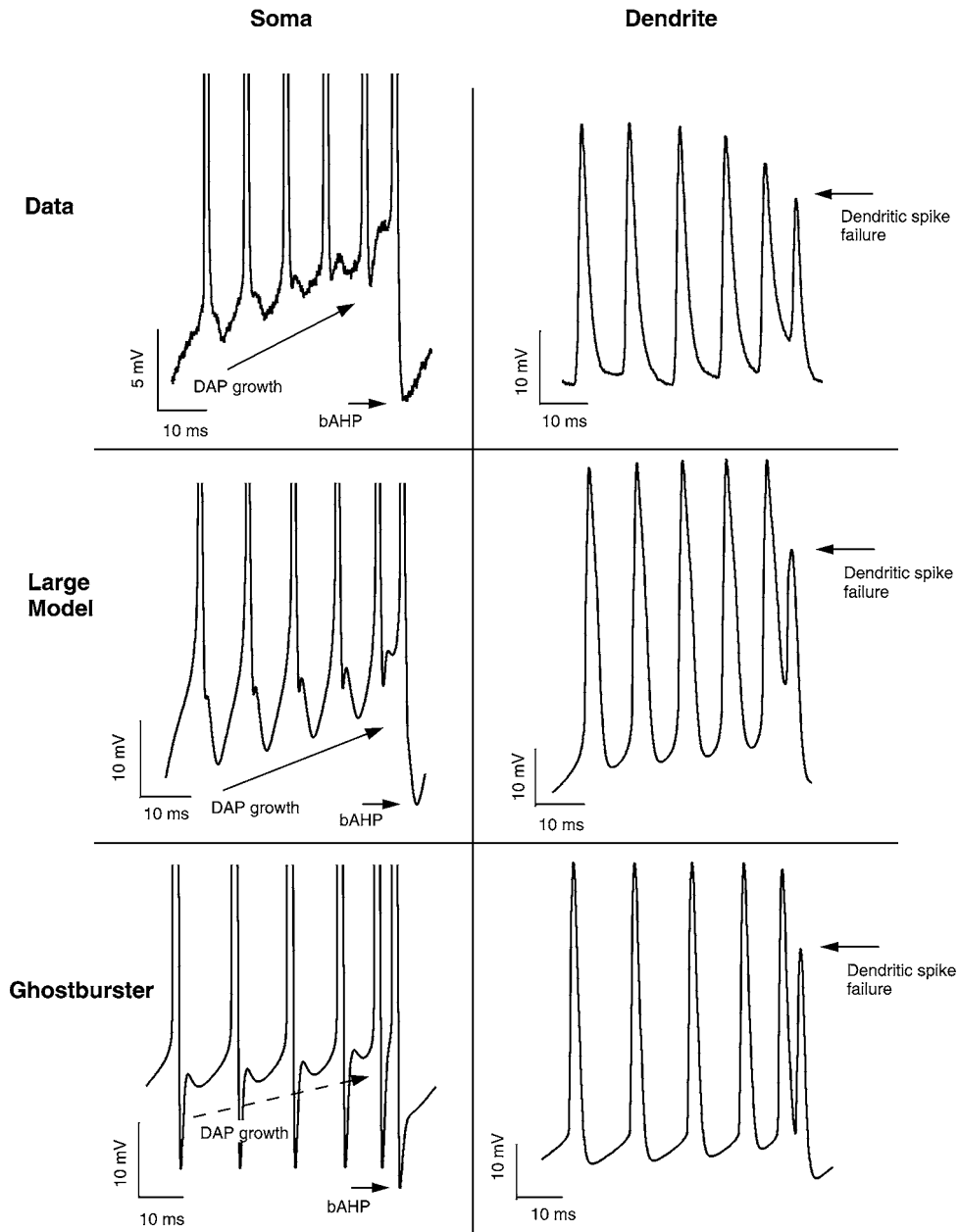
Figure 4. Model performance. A single burst is obtained from ELL pyramidal cell recordings (top row; data donated by R.W. Turner), full multicompartmental model simulations (middle row; simulation presented in Doiron et al., 2001b), and reduced two-compartment model simulations (bottom row; Eqs. (1) through (6)). All bursts are produced by applying constant depolarization to the soma (0.3 nA top; 0.6 nA middle; I_S = 9 , bottom). The columns show both somatic and dendritic responses for each row. The reduced-model somatic spike train reproduces both the in vitro data and full-model simulation spike trains by showing the growth of DAPs and reduction in ISI as the burst evolves. All somatic bursts are terminated with a large bAHP, which is connected to the dendritic spike failure.
