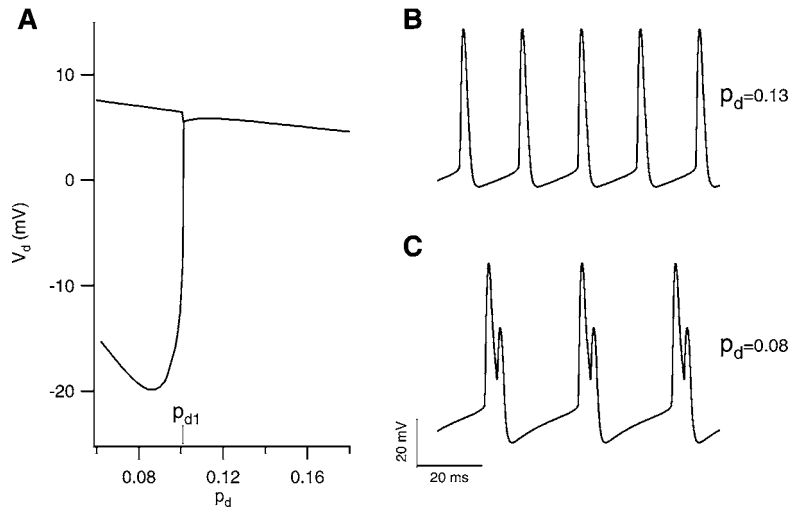
Figure 7. A: Quasistatic bifurcation diagram. p_d is fixed as a bifurcation parameter, while V_d is chosen as a representative variable from the fast-subsystem x . The maxima in the dendritic voltage ( \frac{dV_d}{dt} = 0 and \frac{d^2V_d}{dt^2} < 0 ) are plotted for each value of p_d . At p_d = p_{d1} , the maxima of V_d switch to two values, corresponding to the values taken during each ISI of a period-two solution. B: Time series of the dendritic voltage, V_d(t) , while p_d = 0.13 > p_{d1} . The fast subsystem follows a period-one solution. C: Time series of the dendritic voltage, V_d(t) , while p_d = 0.08 < p_{d1} . The fast subsystem follows a period-two solution. A constant value of I_S = 9 > I_{S1} is chosen for all simulations in A, B, and C.
