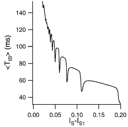
Figure 10. Interburst interval, \langle T_{IB} \rangle is plotted as a function of I_S - I_{S1} . The averaging was performed on 100 bursts produced by the ghostbuster equations at a specific I_S . g_{Dr,d} was set to 12.14. \langle T_{IB} \rangle shows a similar functional form to that described by Eq. (11). The dips in \langle T_{IB} \rangle are discussed in the text.
