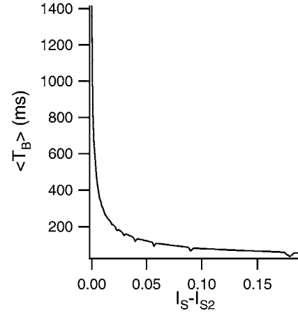
Figure 12. Burst interval \langle T_B \rangle plotted as a function of I_S - I_{S2} . The averaging was performed on 100 bursts produced by the ghostbuster equations at a specific I_S . g_{Dr,d} was set to 12.14. \langle T_B \rangle shows a similar functional form to that described by Eq. (12).
