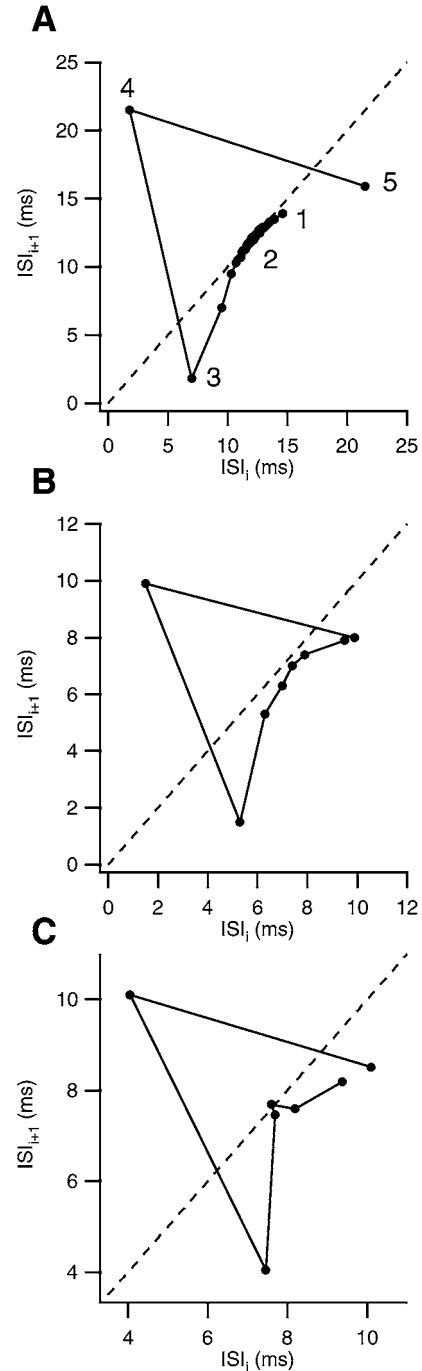
Figure 11. Burst intermittency. A: The ISI return map for a single-burst sequence with I_S = 6.587 and g_{Dr,d} = 13 is shown (for these parameters I_{S1} = 5.736 and I_{S2} = 6.5775 ). The diagonal is plotted as well (dashed line). The labels (1) through (5) are explained in the text. B: The ISI return map for a single-burst sequence with I_S = 9 and g_{Dr,d} = 15 as in Fig. 3. C: The ISI return map for a single-burst recording from an ELL pyramidal cell (data courtesy of R.W. Turner). Compare with the model burst sequence in B.
