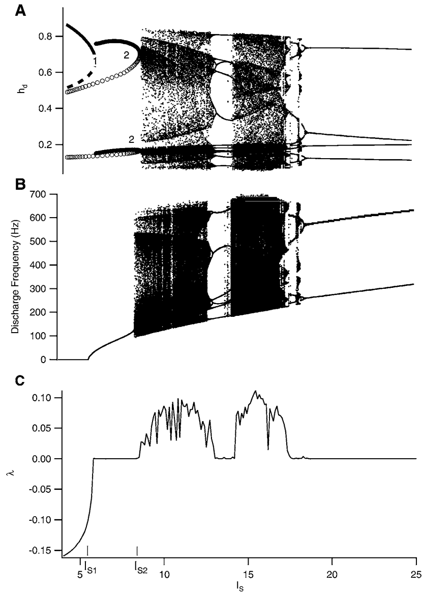
Figure 5. A: Bifurcation diagram of the ghostbuster equations (Eqs. (1) through (6)) as a function of the bifurcation parameter I_S . We choose h_d as the representative dynamic variable and plot h_d on the vertical axis. For I_S < I_{S1} a stable fixed point (solid line) and a saddle (dashed line) coexist. A saddle-node bifurcation of fixed points (SNFP) occurs at I_S = I_{S1} . For I_{S1} < I_S < I_{S2} stable (filled circles) and unstable (open circles) limit cycles coexist, the maximum and minimum of which are plotted. A saddle-node bifurcation of limit cycles (SNLC) occurs at I_S = I_{S2} . For I_S > I_{S2} a chaotic attractor exists; we show this by plotting the maximum and minimum of h_d for all ISIs that occur in a 1 s simulation for fixed I_S . A reverse-period doubling cascade out of chaos is observed for large I_S . The software package AUTO (Doedel, 1981) was used to construct the leftmost part of the diagram. B: Instantaneous frequency ( 1/ISI ) is plotted for I_S simulations of the ghostbuster model for each increment in I_S . The transitions from rest to tonic firing and tonic firing to chaotic bursting are clear. C: The maximum Lyapunov exponent \lambda as a function of I_S .
