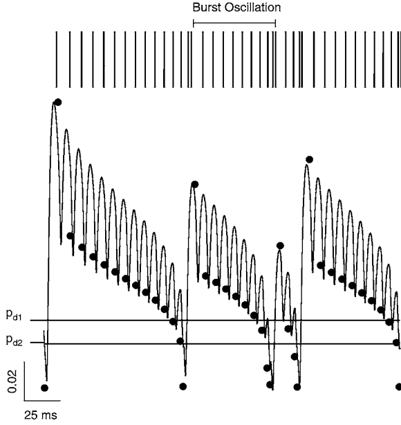
Figure 8. p_d(t) and \tilde{p}_d computed from integration of the ghost-burster equations with I_S = 9 > I_{S2} . Four bursts are shown with the corresponding time-stamped spikes given above for reference. A slow burst oscillation in p_d(t) is observed. It is evident that the discrete function \tilde{p}_d (solid circles) tracks the burst oscillation in p_d(t) . \tilde{p}_d shows a monotonic decrease throughout the burst until the interburst interval, at which point \tilde{p}_d is reinjected to a higher value. The horizontal lines are the values p_{d1} , corresponding to the period doubling transition, and p_{d2} , corresponding to the crossing of the nullcline curve with the \langle V_d \rangle curve. The p_d(t) reinjection occurs after p_d(t) < p_{d2} as explained in the text and in Fig. 9A. \tilde{p}_d has been translated downward to lie on top of the p_d(t) time series. This is required because Eq. (10) uses an unweighted average of V_d , given in Eq. (9). This produces a \tilde{p}_d series that occurs at higher values than p_d(t) because Eqs. (9) and (10) ignore the low-pass characteristics of Eq. (6). However, only the shape of \tilde{p}_d is of interest, and this is not affected by the downward translation.
